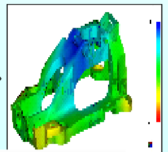
Mold Flow Analysis of Shifter Box
